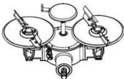
Mechanical unit monoblock with double plate.
